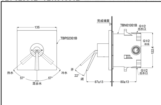
Wall-Mount Mixer Panel/Valve Cartridge TBP02301B+TBN01001B +Univalve Box
